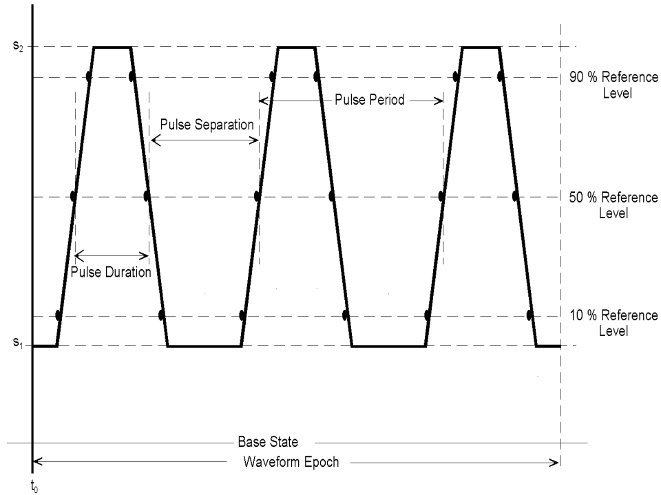
Figure 11—Pulse train
