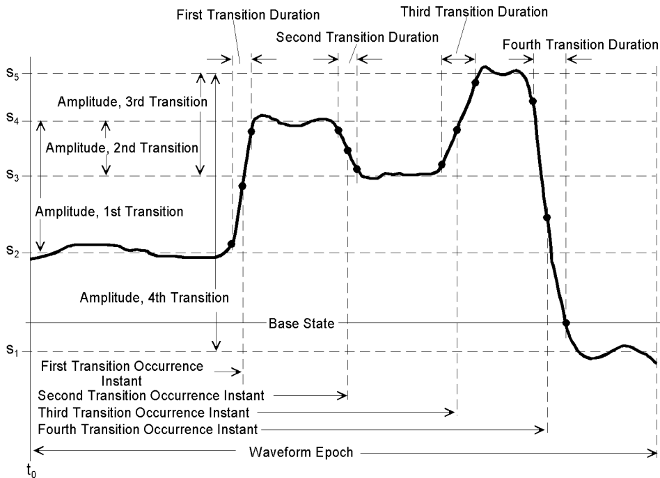
Figure 6—Compound waveform
